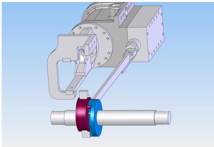
Figure 1 A typical slip eccentric (part of eccentric strap omitted)
